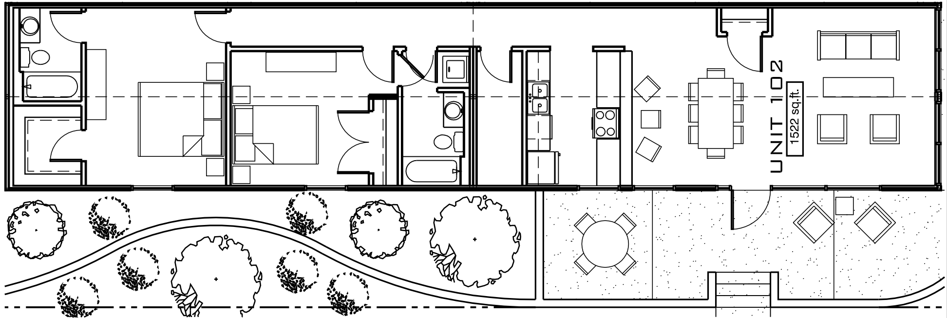
① FLOOR PLAN SCALE: 1/8" = 1'-0" DATE: 15 MAY 2008
