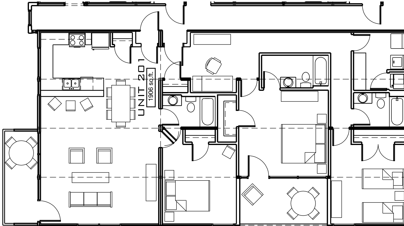
① FLOOR PLAN SCALE: 1/8" = 1'-0" DATE: 15 MAY 2008
