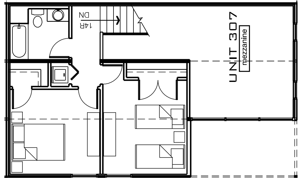
② SECOND FLOOR PLAN SCALE: 1/8" = 1'-0" DATE: 15 MAY 2008
