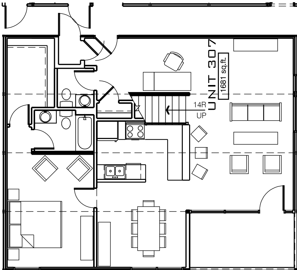
① FIRST FLOOR PLAN SCALE: 1/8" = 1'-0" DATE: 15 MAY 2008
