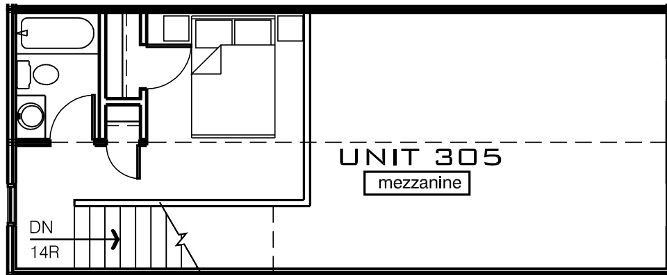
② UPPER LEVEL PLAN SCALE: 1/8" = 1'-0" DATE: 15 MAY 2008
